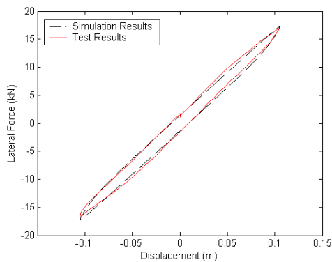
Fig. 11 Hysteresis loop of the air spring in lateral direction, K_{xy} = 154 \text{ kN/m} , K_{yy} = 82.26 \text{ kN/m} , C_y = 1.109 \text{ kNs/m} , k_{haupt} = 96 \text{ kN/m} , C_{haupt} = 1.52 \text{ kNs/m} , \zeta = 0.00063
