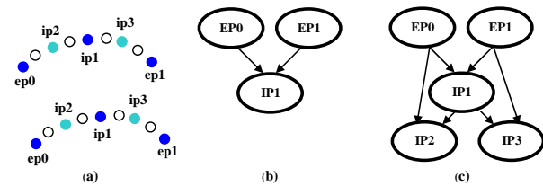
Fig. 1 The recursive construction of a stroke model(a) Example for ip1's: median point of stroke ip2s at ip3's: those of the strokes partial lifts and right, (b) stroke model depth d = 1 , (c) Stroke Model depth d=2
