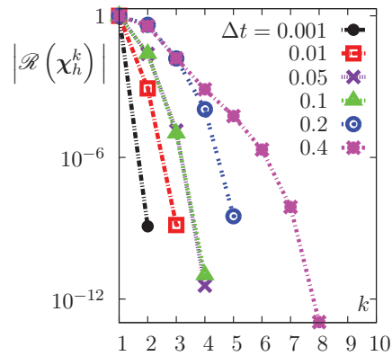
Fig. 4 Convergence curves of the residuals with respect to the Newton iteratis for various time step sizes: Results are plotted in the semi-logarithmic scale
