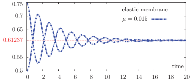
Fig. 3 Temporal evolution of the major and minor axes of the elastic stretched membrane for \mu = 0.015
