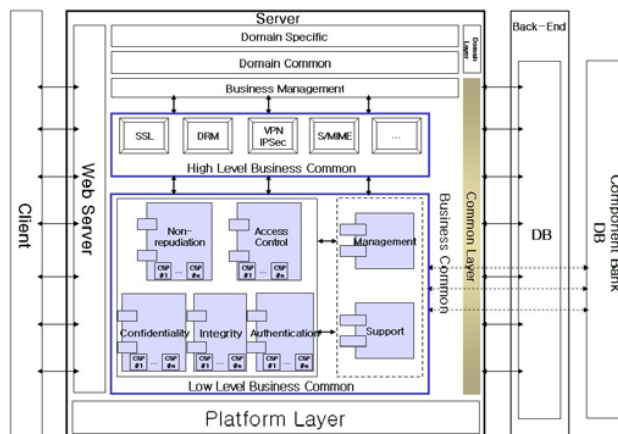
Fig. 1 Information Security Component Framework
