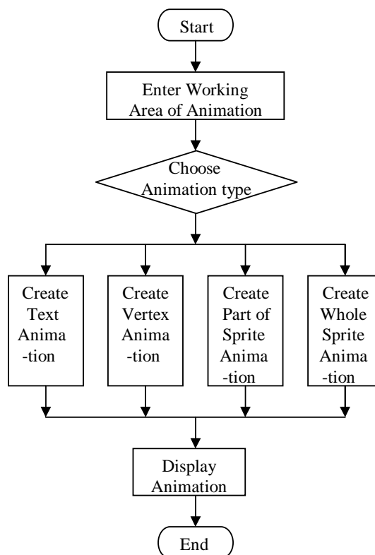
Fig. 1 Overview flowchart of the Animation System
