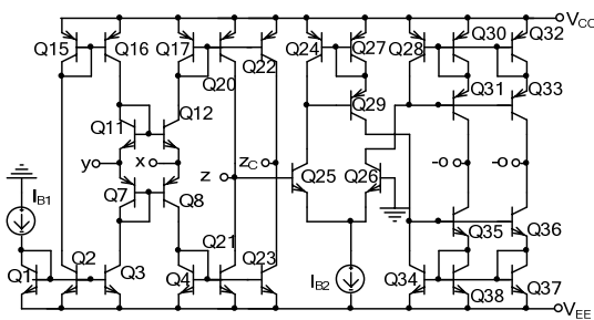
Fig. 3 Internal construction of the BJT CCCCTA
