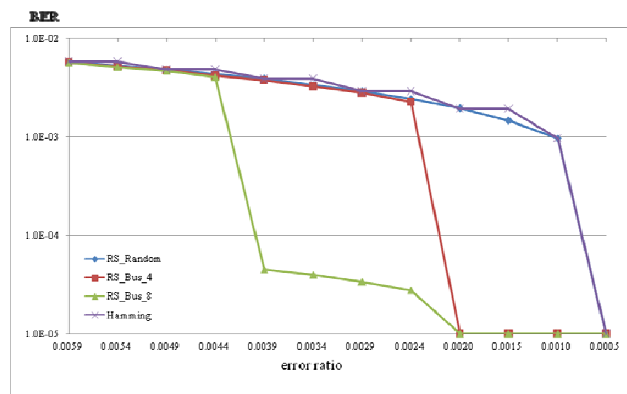
Fig. 7 BER performance for several situations
