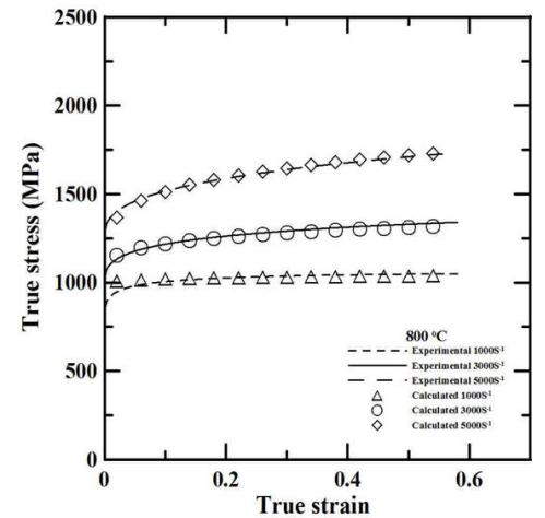
Fig. 3 (c) Comparison of predicted and experimental stress-strain curves for Haynes 188 alloy deformed at temperatures of 800°C
