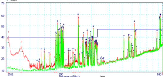
Fig.10 Radiated Emission without a proper filter
