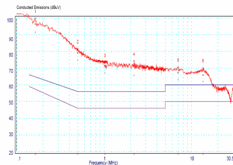
Fig.6 Conducted Emissions without Common Mode Filter
