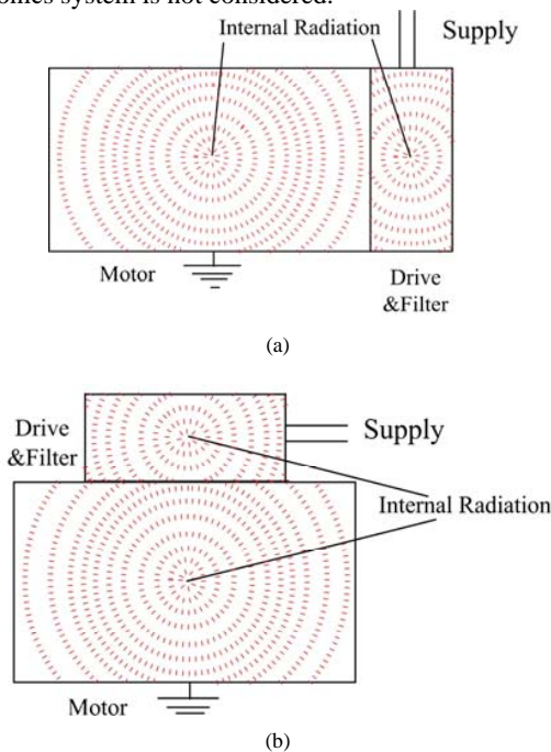
Fig.3 Position of Drive with respect to Motor
