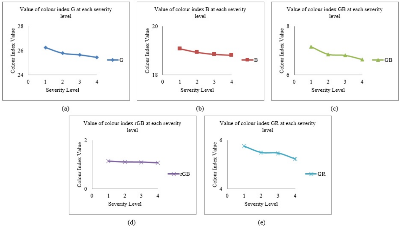
Fig. 2 Relationship between G, B, GB, rGB, GR indices and BSR severity level
