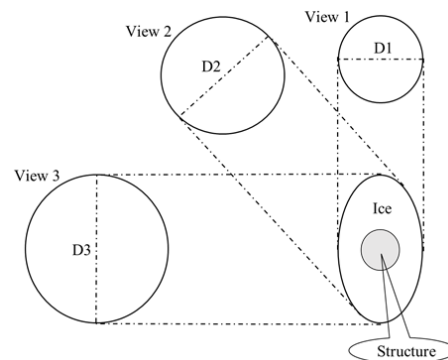
Fig. 4 The schematic of an iced structure with ellipse cross section from different views
