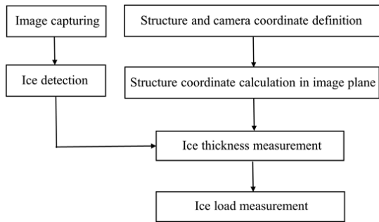
Fig. 2 Block diagram of ice load measurement
