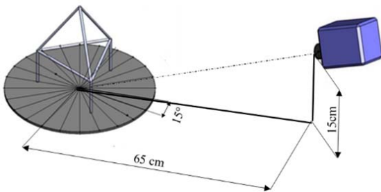
Fig. 6 The schematic of experimental setup
