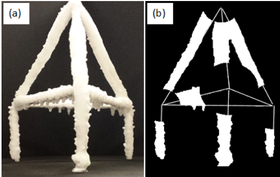
Fig. 9 Image processing results for the structure located at the angle of 165^\circ ; (a) Ice detection results, (b) Removing the joints using the structure scheme
