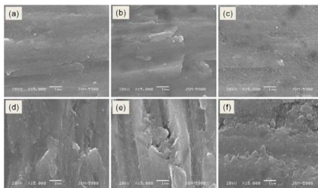
Fig. 2 Various \text{TiO}_2 films grown under different conditions at 200°C (a) 2% \text{I}_2 aqueous solution (b) 2% \text{I}_2 ethanolic solution (c) 2% \text{I}_2 aqueous solution with 1g CTAB (d) 2% \text{I}_2 ethanolic solution with 1g CTAB (e) 2% \text{I}_2 aqueous solution with 1g NaAOT (f) 2% \text{I}_2 ethanolic solution with 1g NaAOT
