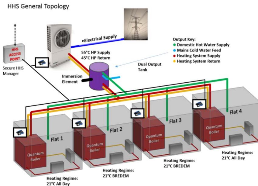
Fig. 9 Schematic of RISE Configuration for MDU
