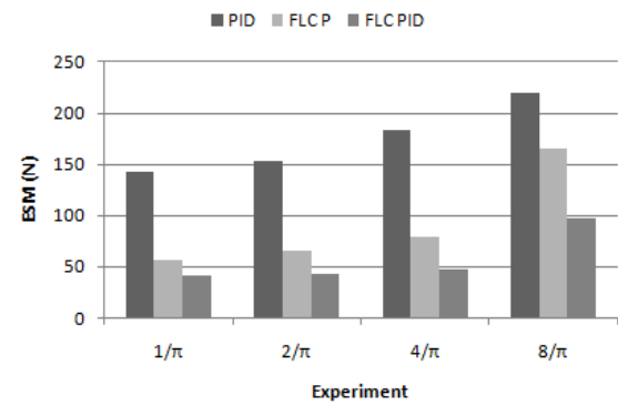
Fig. 17. ESM analysis of several sinusoidal tracking responses – S1.
