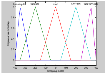
(c) Stepping motor command MFs
