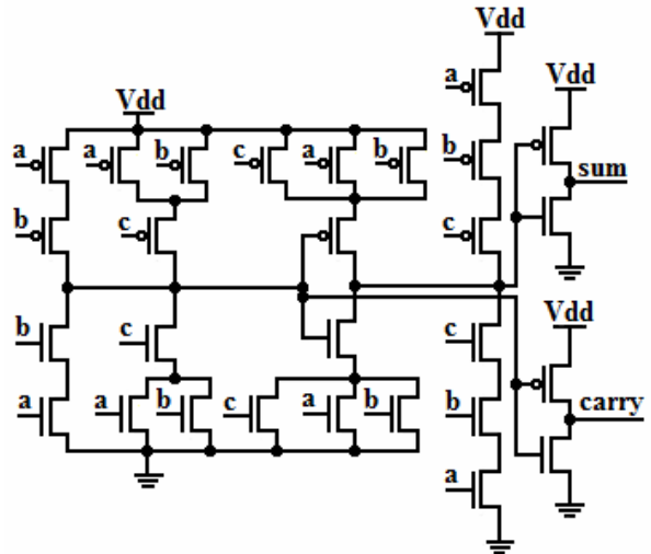
Fig. 3 Conventional CMOS
