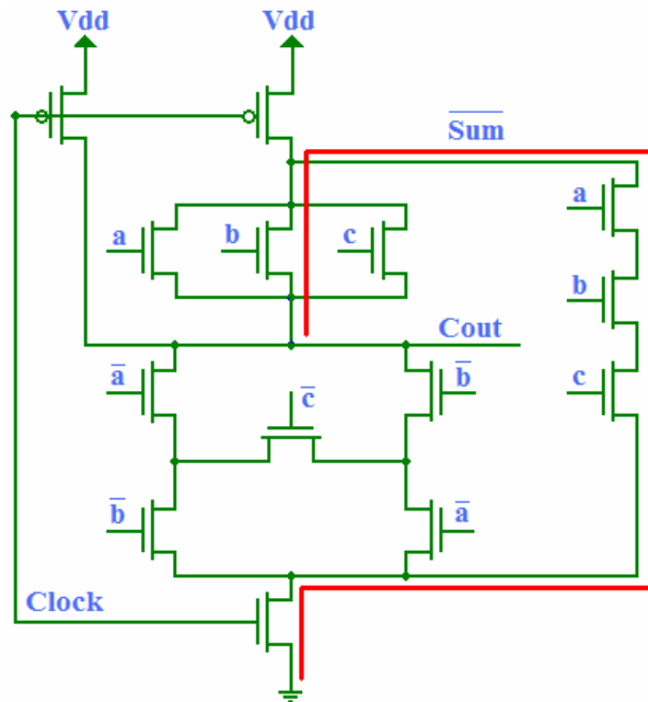
Fig. 8 Primary Schema for the Second Design
