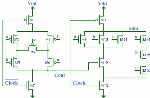
Fig. 7 First Proposed Full Adder Cell Using NP-CMPS Dynamic Logic
