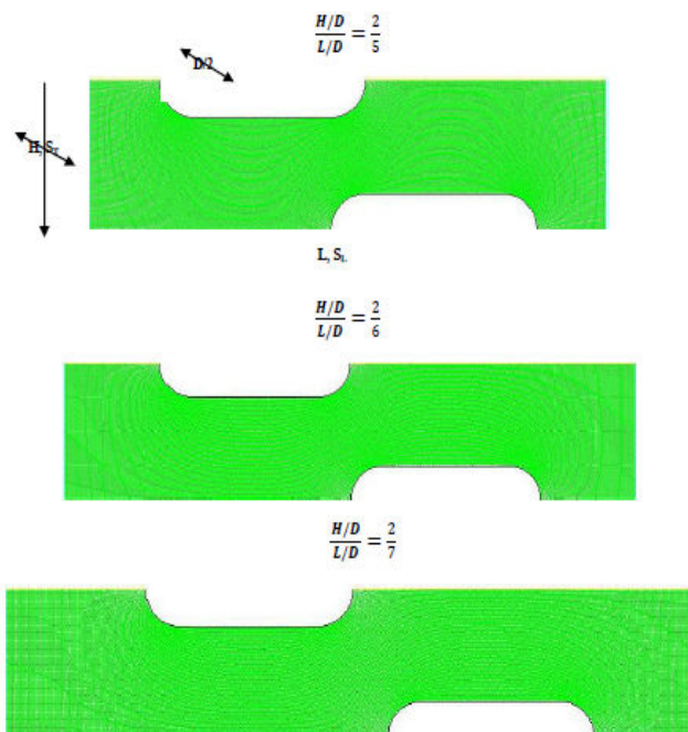
Fig. 1 Grid of laminar flow for Re =400
