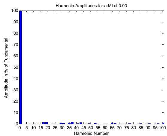
Fig. 8 Harmonic amplitude of 15-level inverter (Modulation index =0.90)
