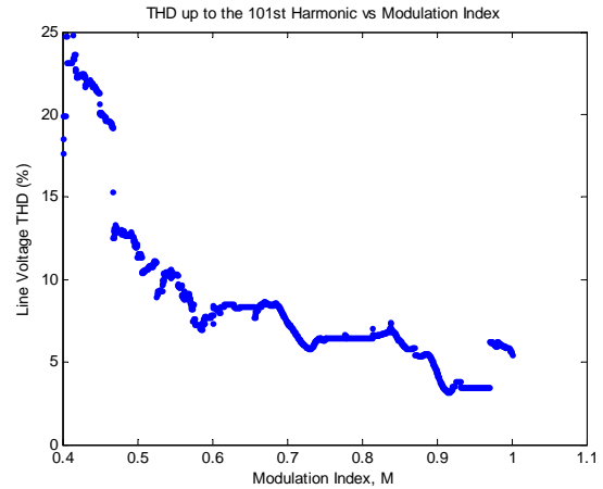
Fig. 7 Line voltage THD versus the modulation index
