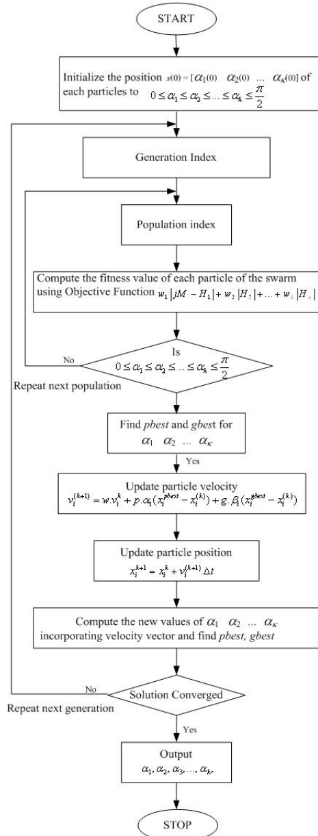
Fig. 4 PSO Flow Chart for calculate switching angle
