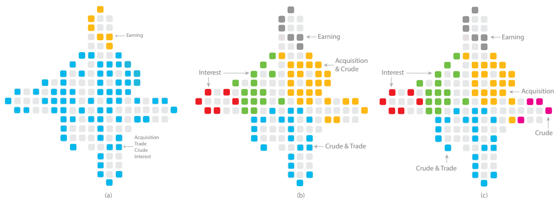
Fig. 5. K-Means based cluster separation (a) K = 2, (b) K = 5, (c) K = 6
