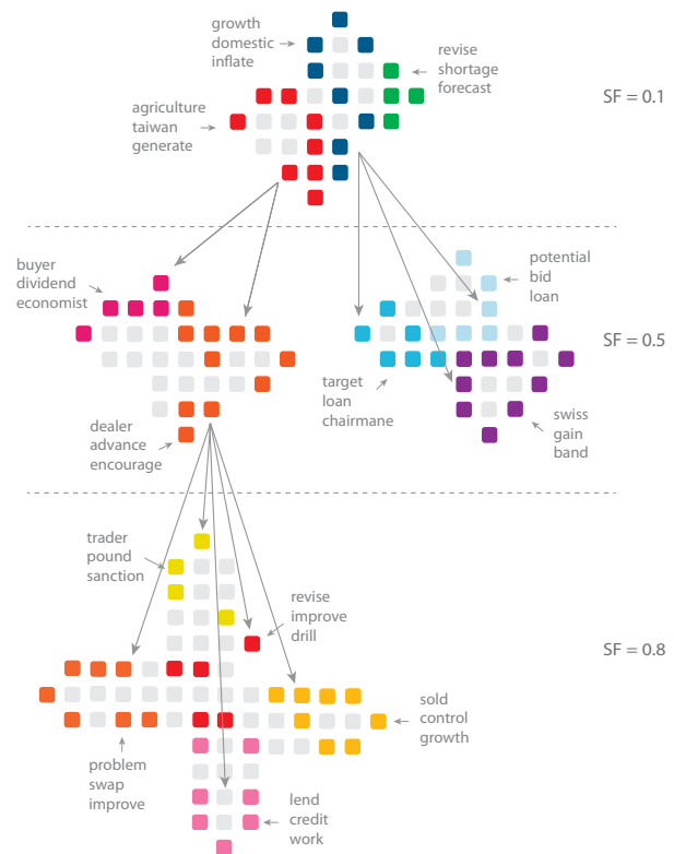
Fig. 8. The GSOM based hierarchical text clustering
