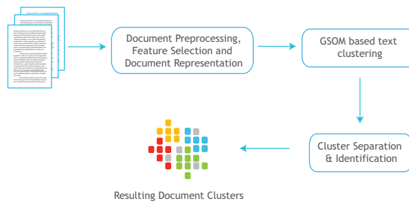
Fig. 3. The GSOM based text clustering model
