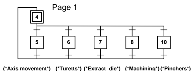
Fig. 5 Page 1 of the Grafset
