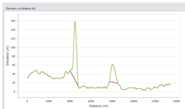
Fig. 5 Elevation profile of the Model Path A
