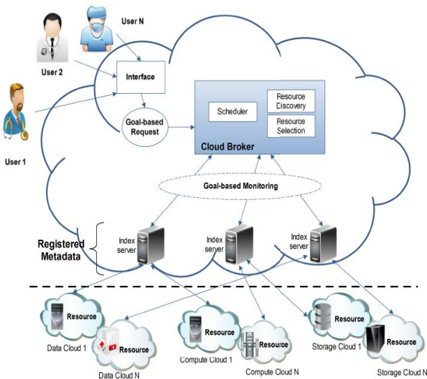
Fig. 5. An overview of cloud resource broker in the medical field.
