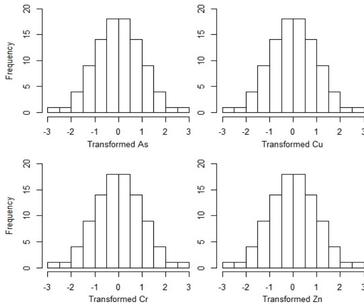
Fig. 2 Histogram of normal-score transformed of As, Cr, Cu and Zn
