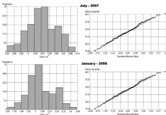
Fig. 6 Histograms and normal QQplots for data, ground-level ozone (ppbV), corresponding to two sampling campaigns
