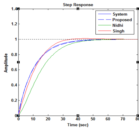
Fig. 2 Comparison of step responses of higher order system, proposed method with previously proposed methods
