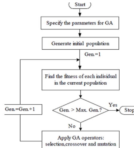
Fig. 1 Flowchart of genetic algorithm [21]
