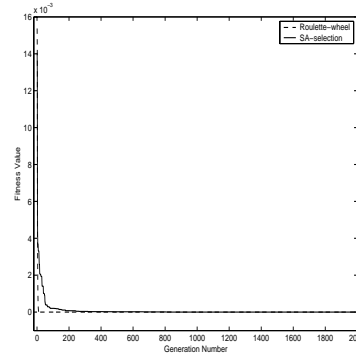
Fig. 6. Convergence of f_A using roulette-wheel and SA-selection
