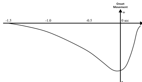
Fig. 1 A typical readiness potential
