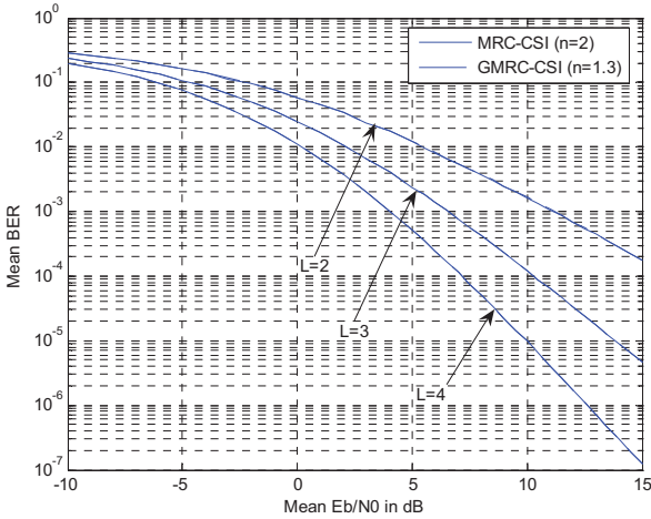
Fig. 3 BER for MRC ( n=2 ) and GMRC ( n=1.3 ) in a Rayleigh fading environment ( P_{dif}=1 ) with perfect channel estimation for 2, 3 and 4 diversity antennas
