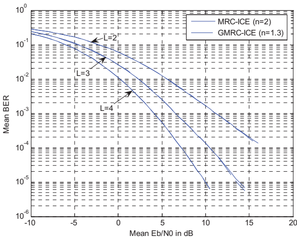
Fig. 4 BER for MRC ( n=2 ) and GMRC ( n=1.3 ) in Rayleigh fading environment ( P_{dif}=1 ) with imperfect channel estimation ( \sigma_E=0.01 ) for 2, 3 and 4 diversity antennas
