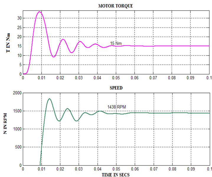
Fig. 6 Transient response of speed and torque at t=0.05\text{sec} for 9-phase induction motor drive
