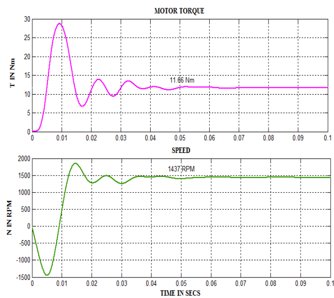
Fig. 5 Transient response of speed and torque at t=0.04\text{sec} for 7-phase induction motor drive
