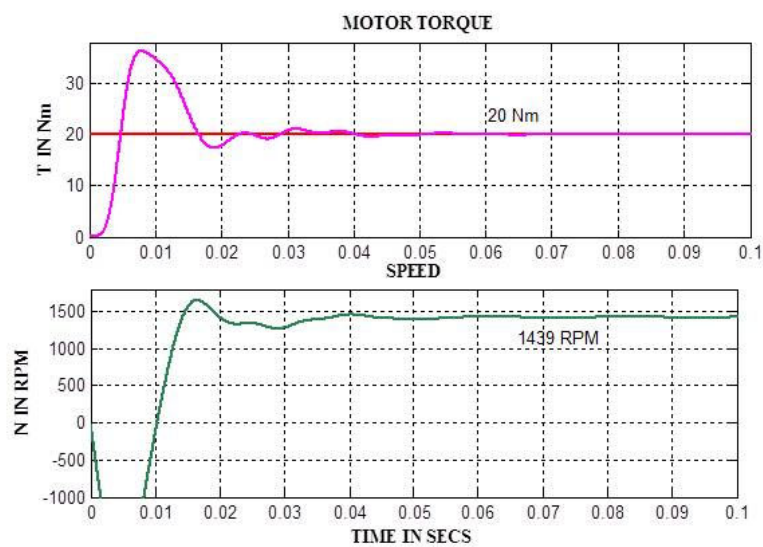
Fig. 7 Transient response of speed and torque at t=0.04\text{sec} for 12-phase induction motor drive
