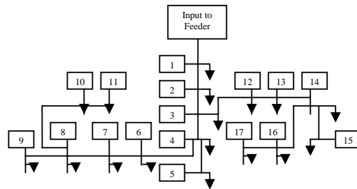
Fig. 2 16-bus test system
