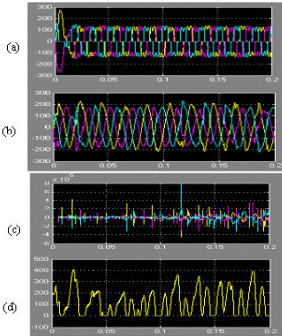
Fig. 5 Fuzzy tuned PID controller based APF simulations under nonlinear and unbalanced load (firing angle of thyristor bridge set at 1200) (a) Is without APF, (b) Is with APF, (c) Compensation current and (d) DC side capacitor voltage
