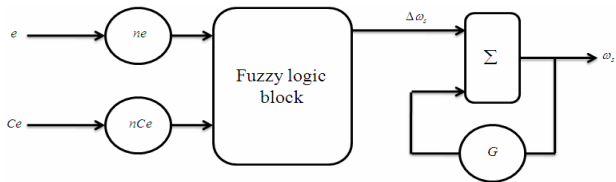
Fig. 2. Structure of fuzzy controller
