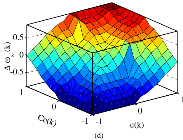
Fig. 3. The memberships of the: a - Error, b - Error variation, c - Command variation, d - Control surface.
