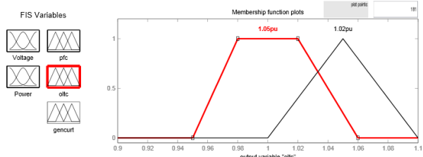
Fig.7 On Load Tap Changer (OLTC) membership functions
