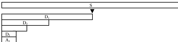
Fig. 4. Wavelets transform of a sequence s .
