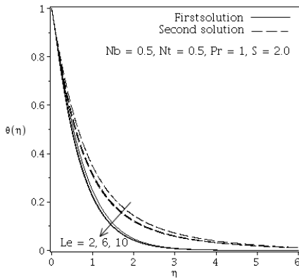
Fig. 1 Effect of Le number on temperature distribution for selected values of Nb , Nt , Pr and S when \varepsilon = -1 (shrinking case)
