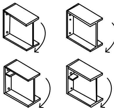
Fig. 1 Typical configurations for flush end-plate
