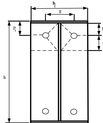
Fig. 9 Yield Line pattern for flush end plate connection
