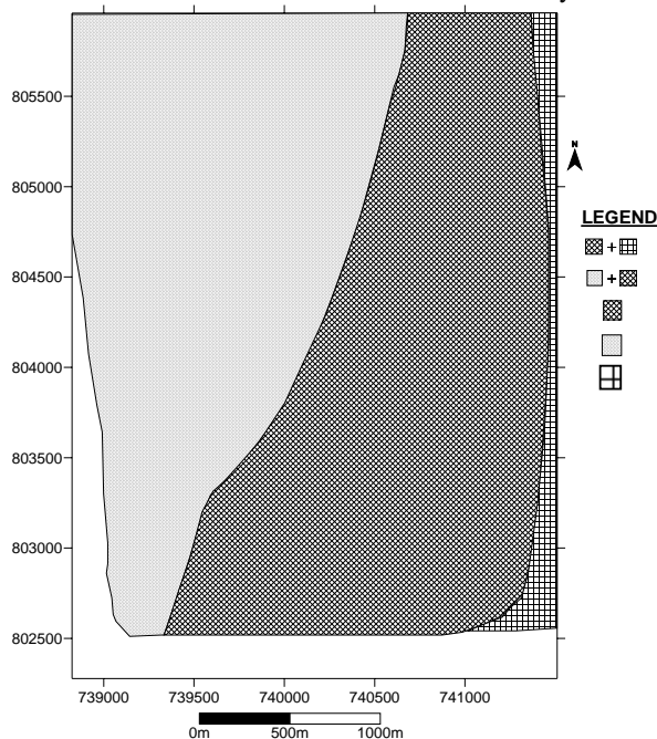
Fig. 10: Proposed model of the emplacement of the charnockitic and associated granitic rocks in the study area.
