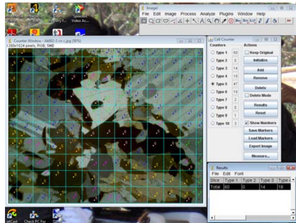
Cell Counter Legend Type 1 is plagioclase, Type 2 is Orthoclase, Type 3 is quartz, Type 4 is Biotite, Type 5 is Hornblende, Type 6 is Mymerkite, Type 7 is Hypersthene, Type 8 is Muscovite and Type 9 is Pyroxene.
