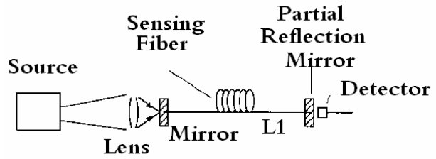
Fig. 7 Fabry-Perot interferometer-based fiber optic sensor
