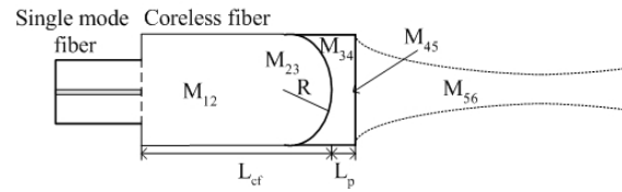
Fig. 1: The proposed fiber lens structure.
