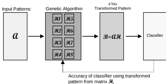
Fig. 3 GA-based feature extractor using an objective function based on classification accuracy. Each transformation matrix from the GA population is used to transform the input patterns, which are then passed to a classifier. The fitness of the matrix is based on the classification accuracy attained on the transformed patterns [15]
