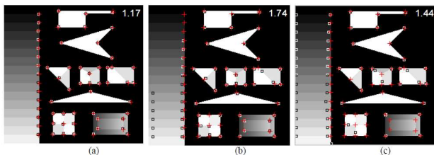
Fig. 10 Comparison of corner localization error using (a) proposed CF corner, (b) impHarris corner, and (c) impCSS corner, where the squares represent the detected corners and the crosses (+) represent the ground truth locations
