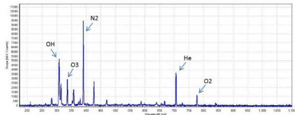
Fig. 6 Optical Emission Spectroscopy
