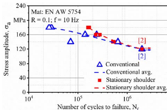
Fig. 10 Woehler curve for fatigue life assessment of welded specimens
