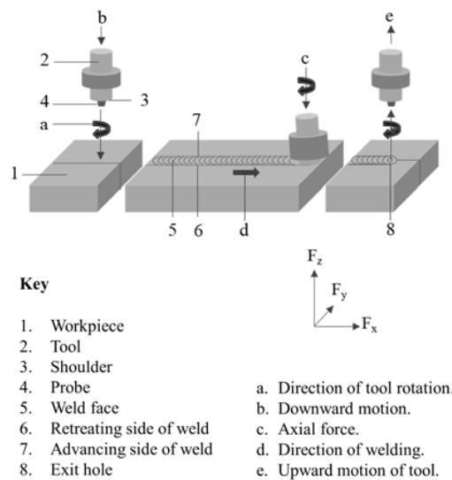
Fig. 1 Operating principle and components of conventional FSW
