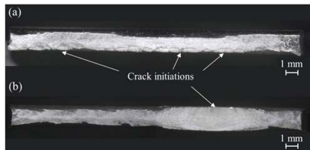
Fig. 13 Light micrograph of the fracture surface of the sample manufactured by (a) conventional and (b) stationary shoulder setup
