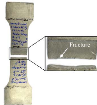
Fig. 12 Example of a fractured specimen at the end of the fatigue tests
