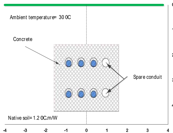
Fig. 19 Duct bank Installation
