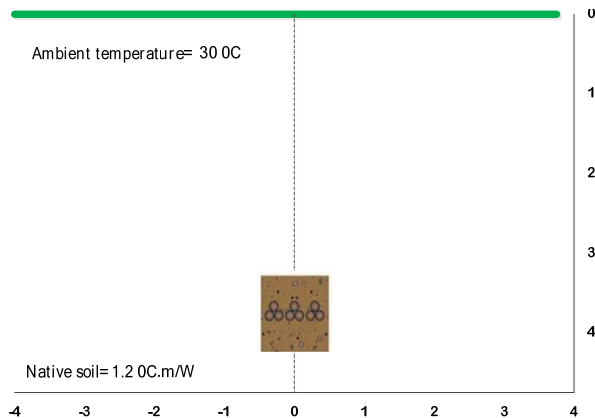
Fig. 20 Three trefoils directly buried in the soil
