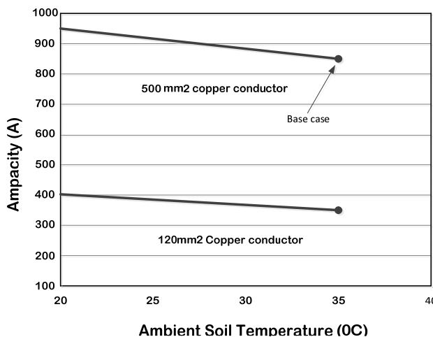
Fig. 8 Ampacity ratings versus ambient soil temperature
