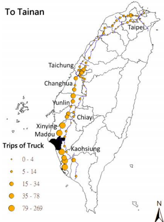
Fig. 10 Truck trips number on Saturdays and Sundays
