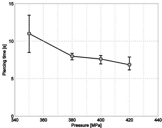
Fig. 4 Effect of water pressure on piercing time
