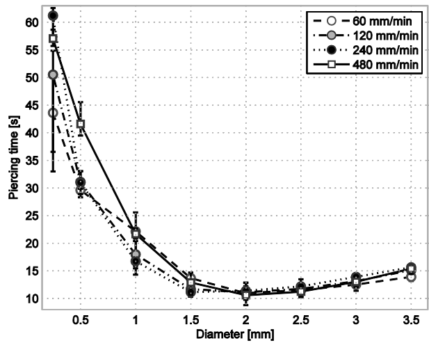
Fig. 11 Piercing times as a function of diameter of circular piercing
