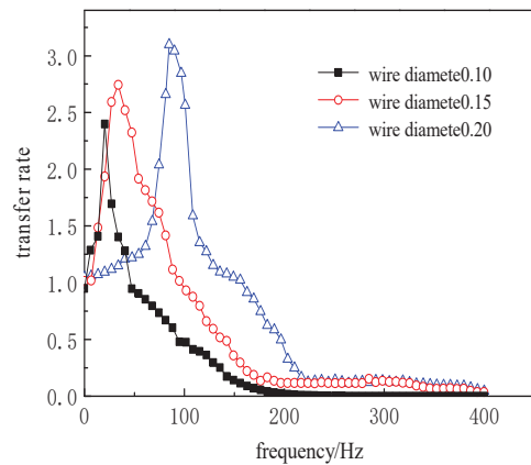
Fig. 9 Transfer rate-frequency curve of different wire diameters
