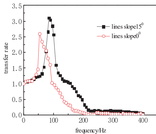
Fig. 5 Transfer rate-frequency curve of different lines slope
