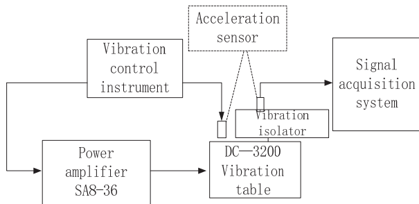
Fig. 4 Schematic diagram of vibration experiment
