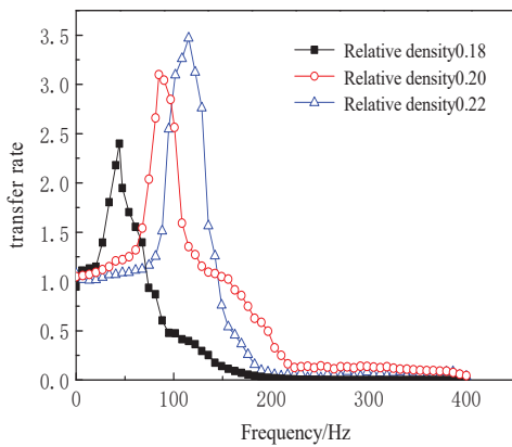
Fig. 7 Transfer rate-frequency curve of different relative densities
