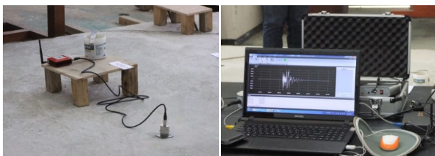
(a) Accelerometer (b) Data measurement
