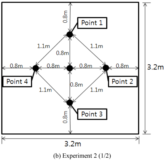
Fig. 2 Point of vibration measurement
