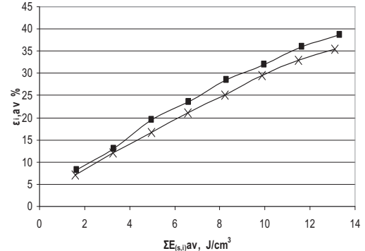
Fig. 7 \Sigma E_{(s,i)av} - \epsilon_{i,av} function by upsetting; ■- controlled impact; x – simple impact
