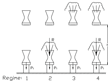
Fig. 3 Regimes of the experimental set-up: 1 – simple impact; 2 – simple impact + controlled impact; 3 – accelerated by rocket engine simple impact; 4 – accelerated impact + controlled impact; P_1 – impact force; R – rocket engine thrust
