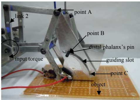
Fig. 3 Robotic finger during final pinching configuration
