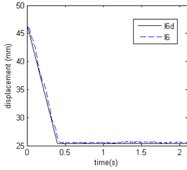
Fig.10 Slider displacement, l_6 under PID control
