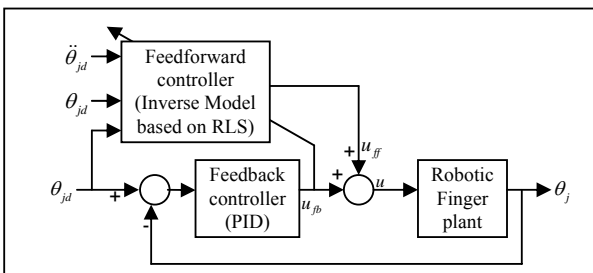
Fig. 5 RLS based FEL control scheme
