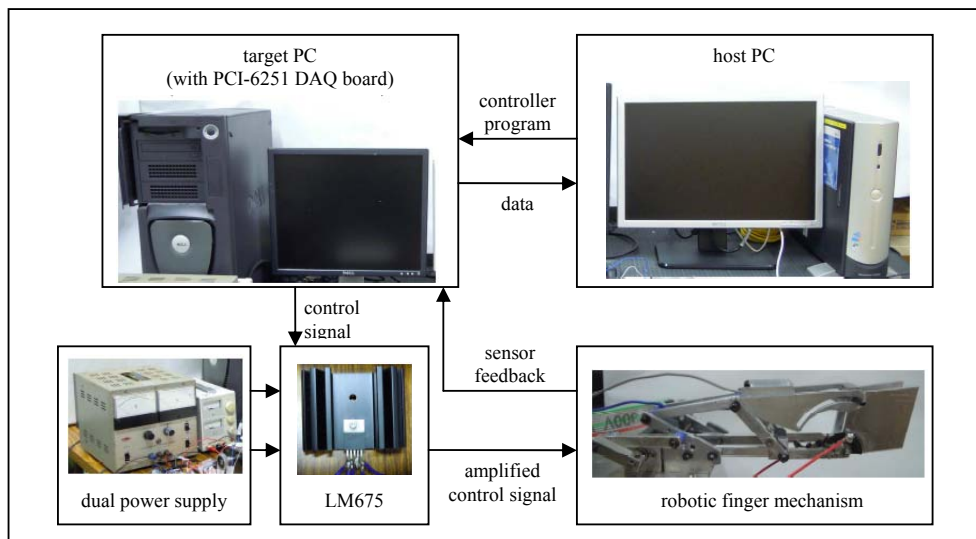
Fig. 6 Hardware set up
