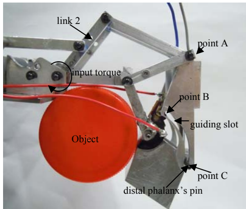
Fig. 2 Robotic finger during final grasping configuration
