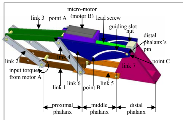
Fig. 1 Finger mechanism (add label no link)
